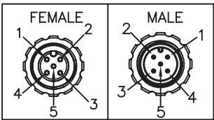
PIN ASSIGNMENTS FRONT VIEW
