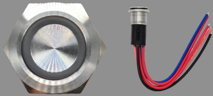
Wire Length: 6" # Of Wires: 5 LED Color: Green Button: SS w/ Translucent Ring 9150-1102-506 (On/Off)
