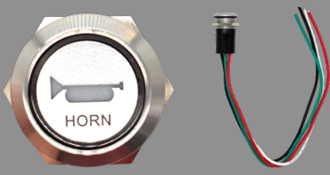
Wire Length: 6" # Of Wires: 4 LED Color: Red Button: SS w/ Translucent Ring 9052-2009-106 9052-2009-106-4 (W/DTM06-4S)
