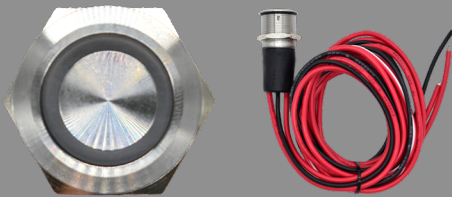
Wire Length: 5' # Of Wires: 3 LED Color: Blue Button: SS w/ Translucent Ring 9050-1014 (On/Off)
