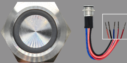
Wire Length: 6" # Of Wires: 5 (DTF) LED Color: Red Button: SS w/ Translucent Ring 9150-2101-506-DTF (Momentary)
