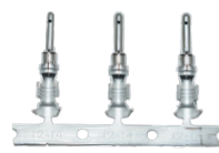
DTP Crimp (12-14) 1060-12-0166
