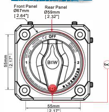
Front Panel Mounting
