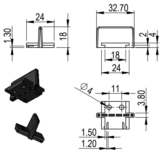
30A Terminal Block Part A 16000-01-0A
