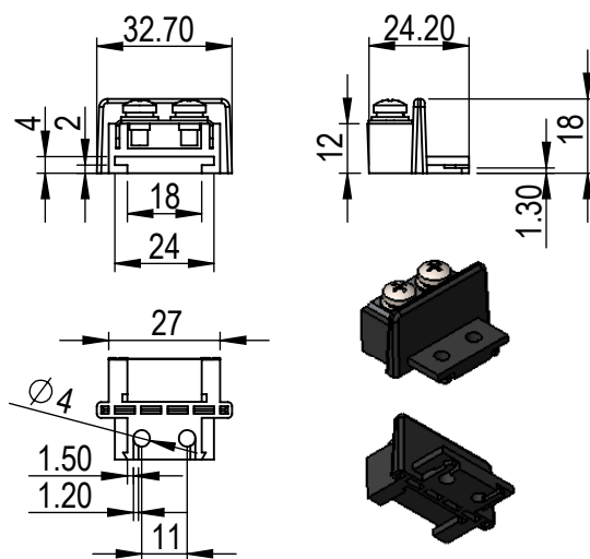
30A Terminal Block Part B 16000-02-0B
