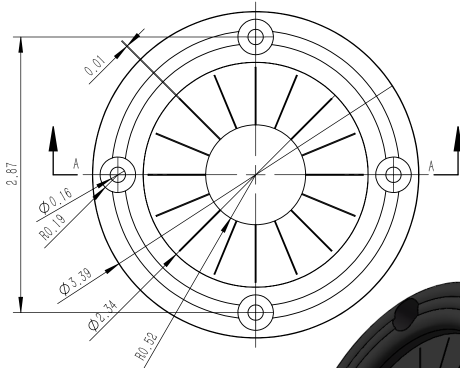
Utility Grommet 3.4" Part No.:1301534-0092
