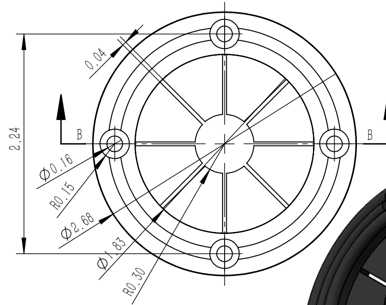
Utility Grommet 2.6" Part No.:1301526-0092
