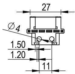
30A Terminal Block Part B 16000-02-0B
